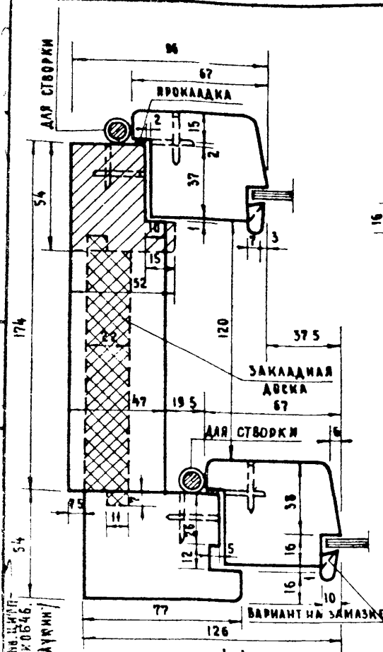
ПО 4-4
