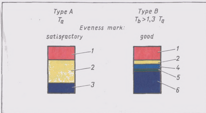
Fig. 6. Indices of the surfacing service life and evenness when constructing the traditional road pavement (Type A) and the road pavement with plastic foam (Type B): 1 — surfacing and base courses of road pavement; 2 — sand; 3, 6 — soil; 4 — Styrofoam; 5 — geotextile
