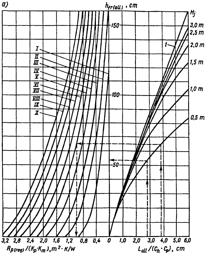
Fig. 11. Nomogram for determining the required thermal resistance of road pavement 1- X — isoline numbers on the map (Fig. 10); 1 — design curve for types 1
